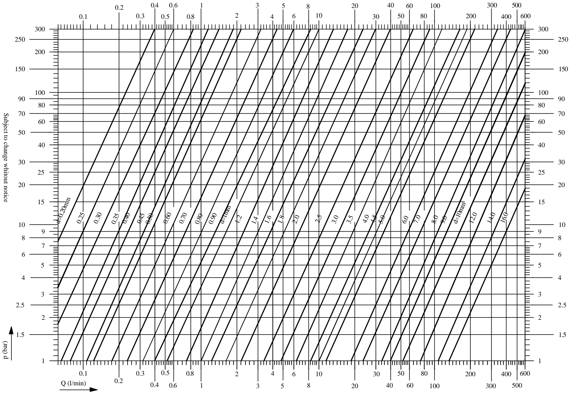
Pressure drop for turbulent flow through a round, sharp-edged, orifice as a function of rate and diameter
