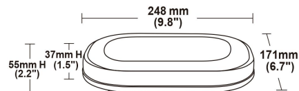
Magnet base
