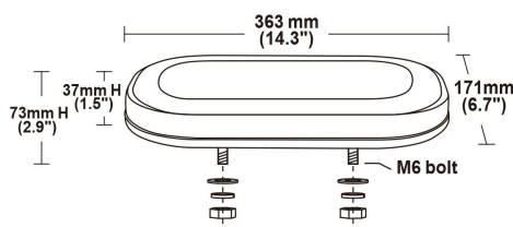
Two bolts base
