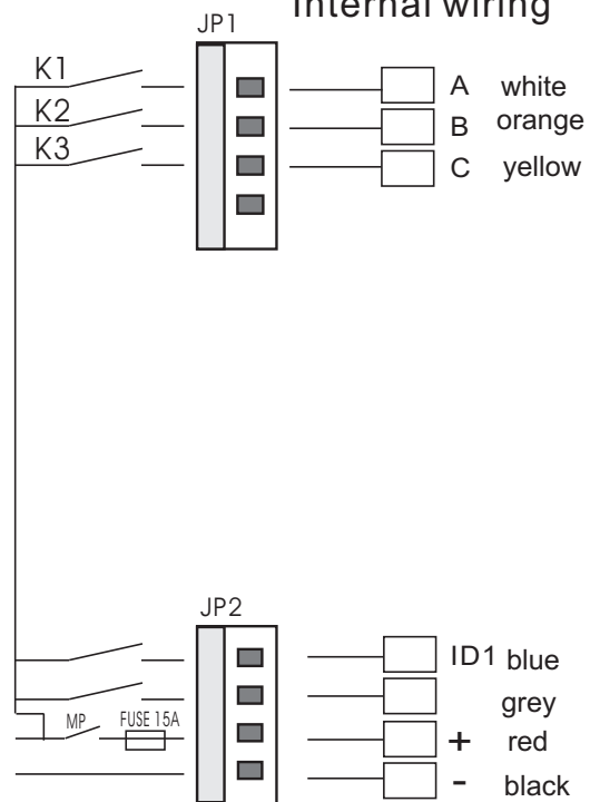
Internal wiring
