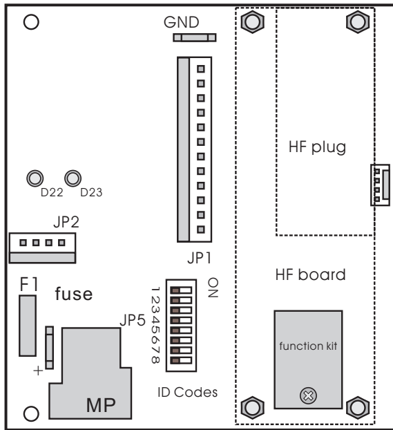
encoder board
