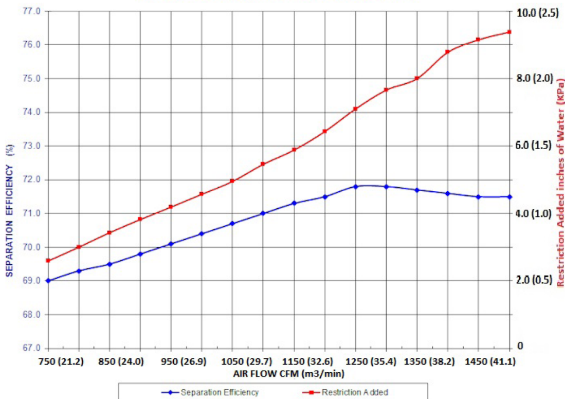
Power Ram Precleaner 5", 6", 7", 8" Separation Efficiency and Restriction Added Curve
