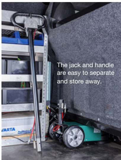
Transportable jack with an exceptionally long reach of 1800 mm.
