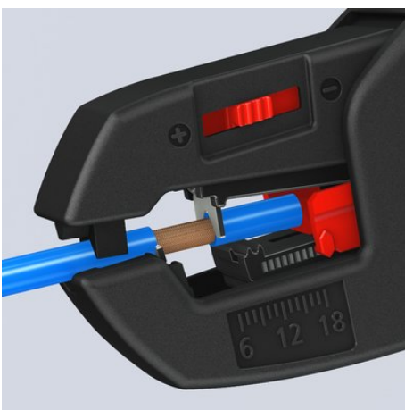
Adjustable length stop, with scale
