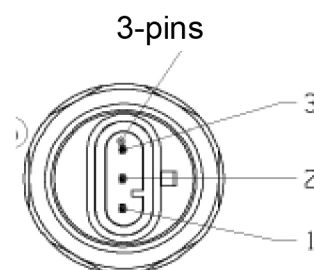
VIEW X
