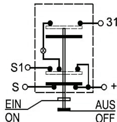
Circuit diagram
