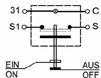
Circuit diagram
